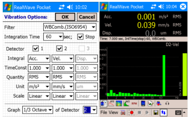
Ship Vibration Setup
