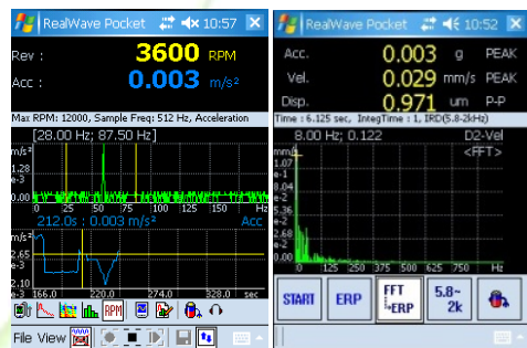
RPM & Vibration Measurement
